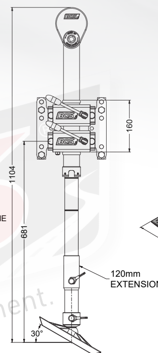
MAXIMUM EXTENSION WITH 120mm EXTENSION & BASE PLATE
