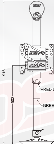
MAXIMUM EXTENSION WITH BASE PLATE
