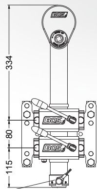
TRAVEL POSITION WITH-OUT BASE PLATE
