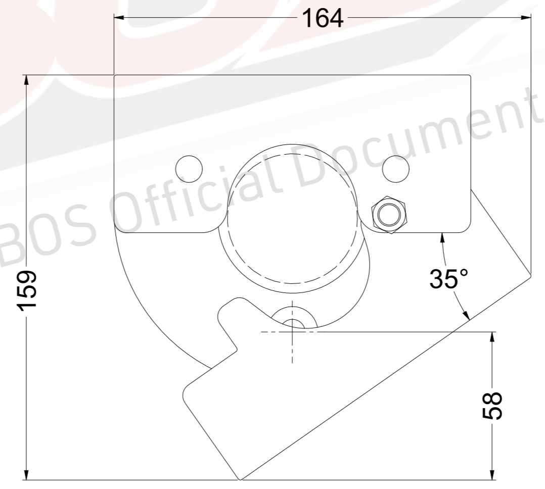
Minimum clearance required to fit Jockey Unit when Clamp is opened
