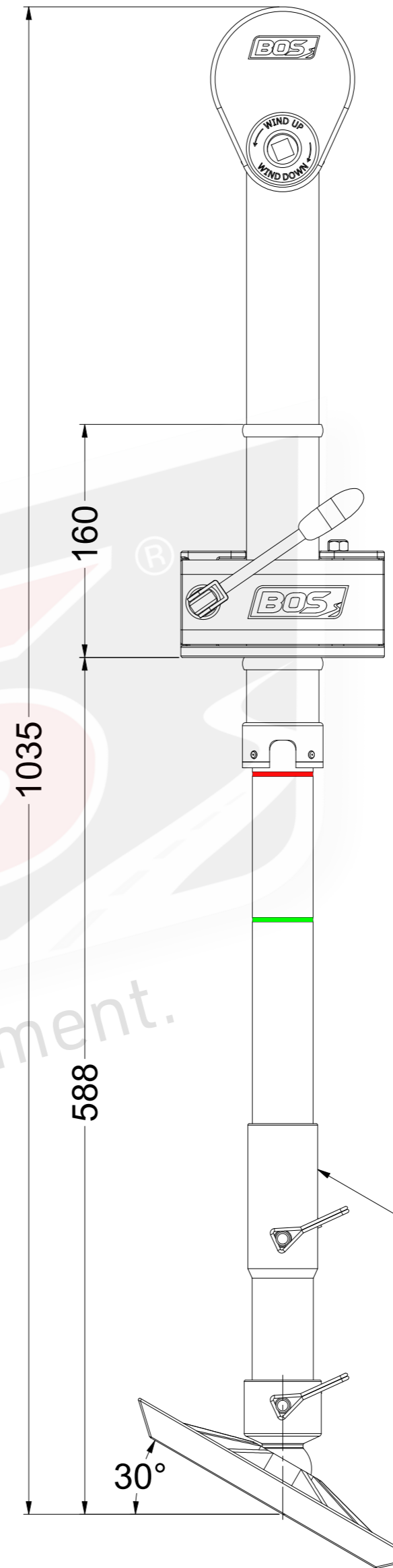
Maximum Extension with 120mm Extension & Base Plate
