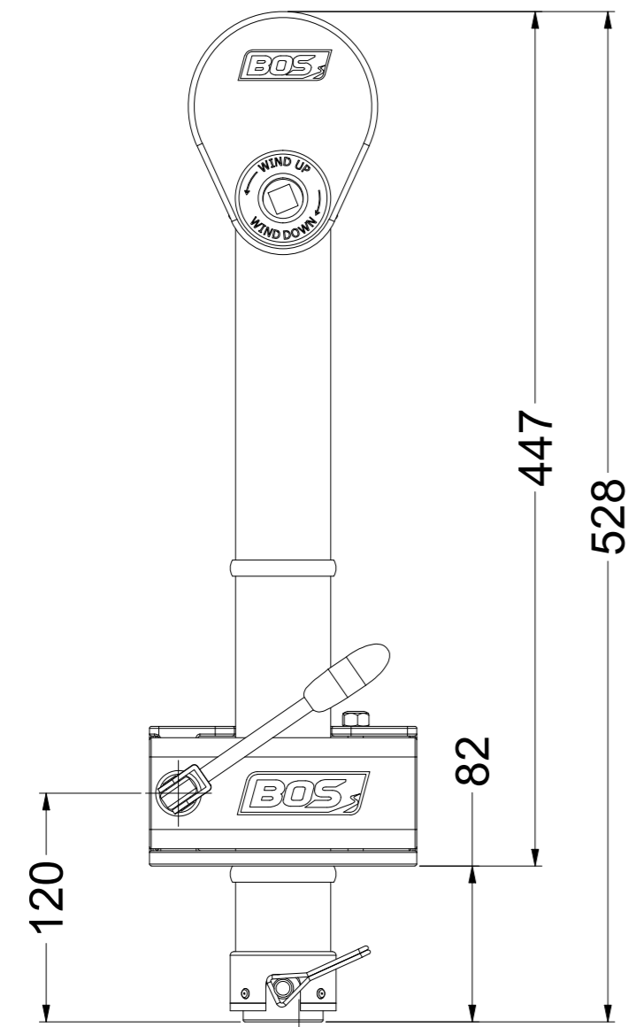
Travel Position without Base Plate
