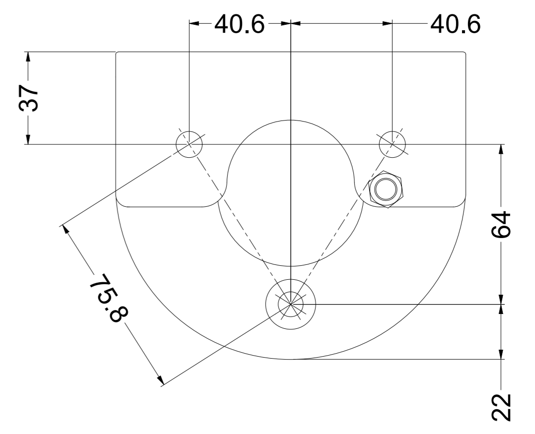
Mounting Holes Detail
