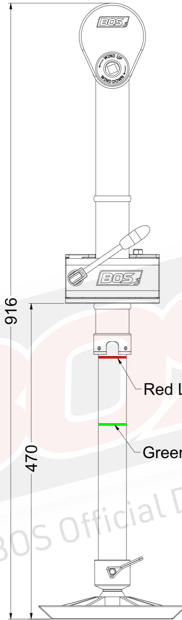
Maximum Extension with Base Plate
