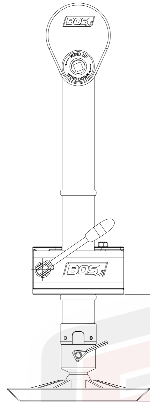
Retracted with Base Plate
