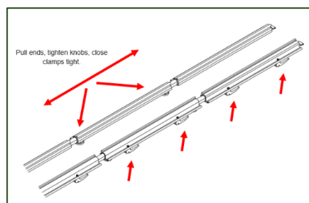
Fig. 11: Tighten knobs and close clamps.
