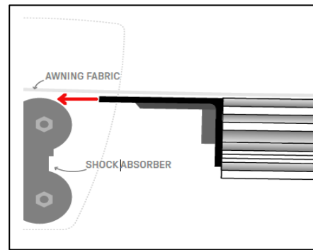
Fig. 8: Paddle end on shock absorber.
