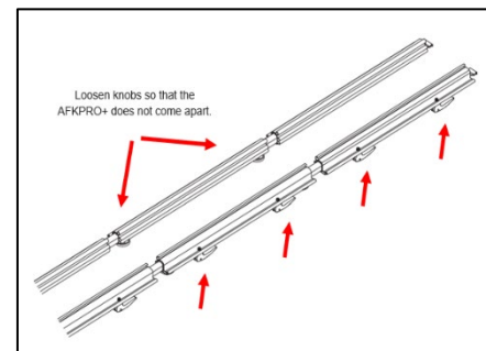
Fig. 9: Loosen Knobs and Open Handles.
