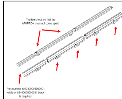
Fig. 2: Knobs and handles
