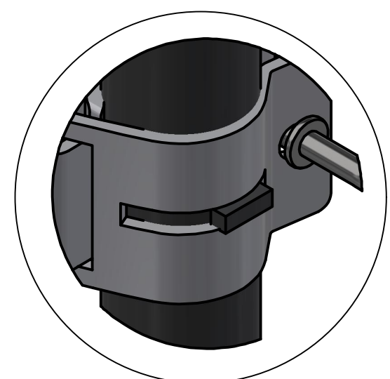
LUG IN CENTRE OF Ø60mm CLAMP
