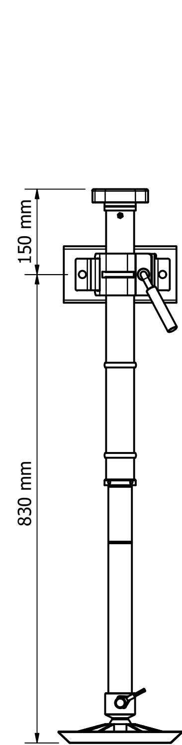
MAXIMUM LIFT
